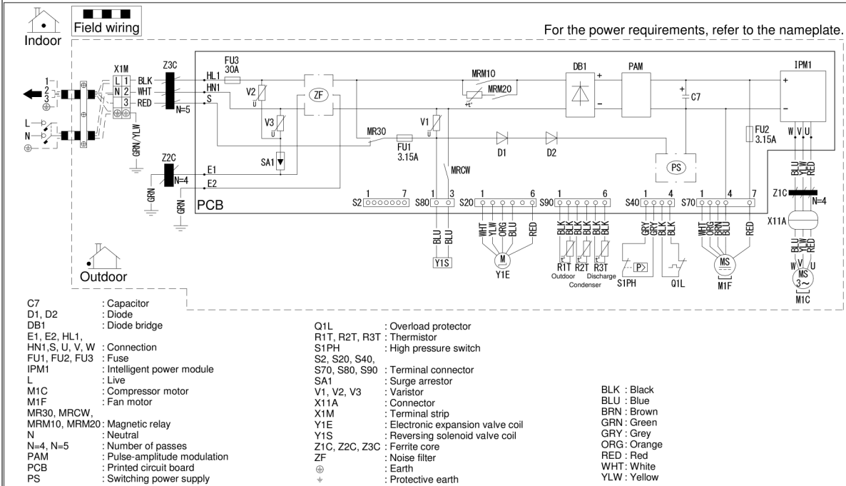
Wiring diagram
