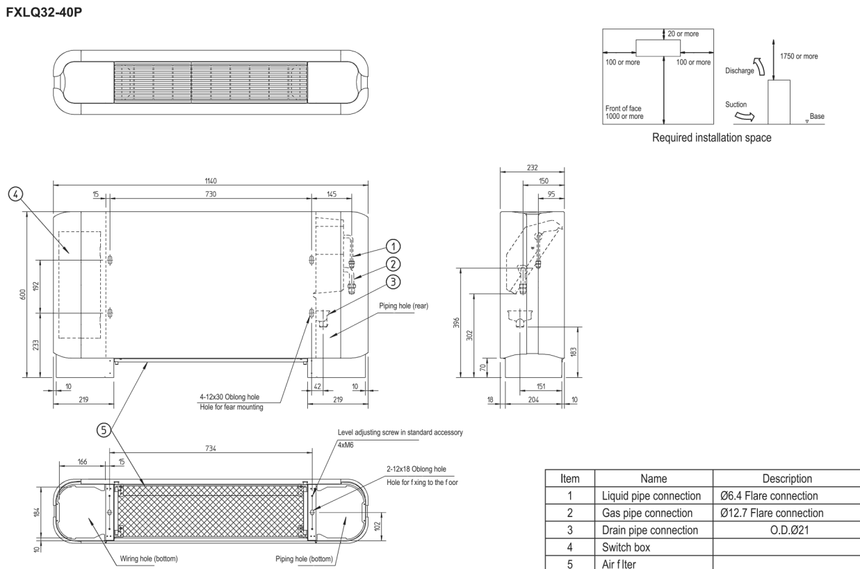
FXLQ32-40P
