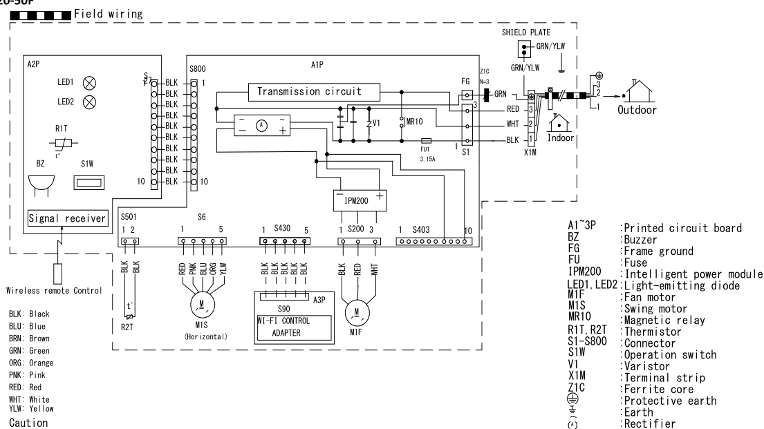
Wiring diagram
